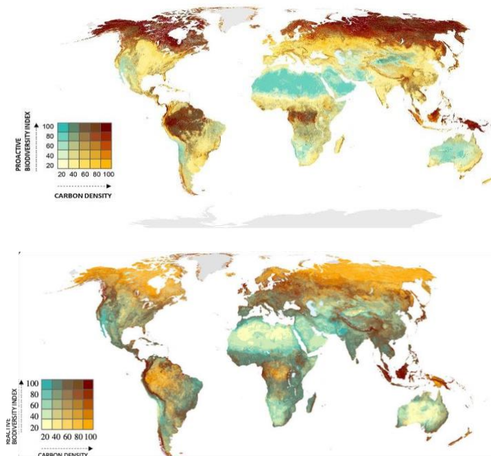
Figure 2. The top map depicts the area of overlap between areas of high local biodiversity (high species richness, range-size rarity), high local intactness and high average habitat condition with carbon-richness. The bottom map depicts the area of overlap between areas of high local biodiversity, low average habitat condition and high threats with carbon richness. The dark brown areas depict the areas of highest overlap. Reprinted with permission 22 .
