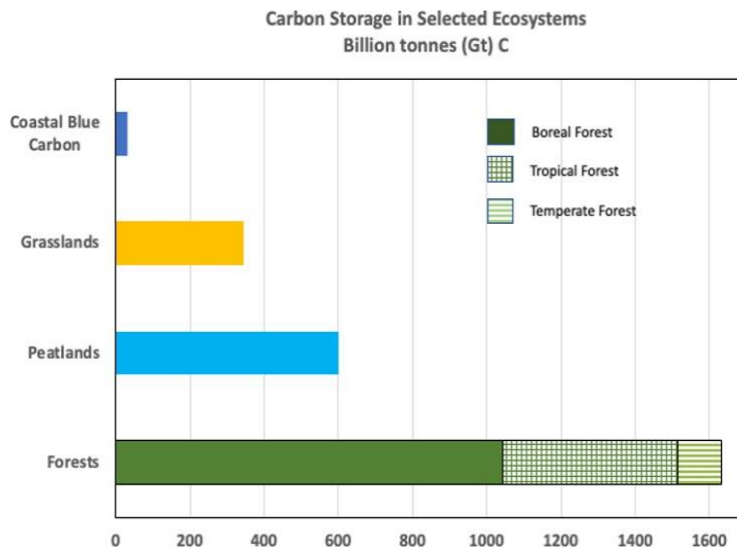
Figure 1: Estimates of global carbon storage in selected ecosystems. Sources for estimates are: Coastal blue carbon (mangroves, salt marshes and seagrass beds) 18 (Macreadie et al 2021); Grasslands 19 (Lorenz and Lal 2018); Peatlands 20 (Strack et al. 2022); Forests 21 (Woods Hole Climate Research Center et al 2020).
