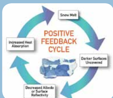
Black carbon: Positive feedback cycle © Oceana
