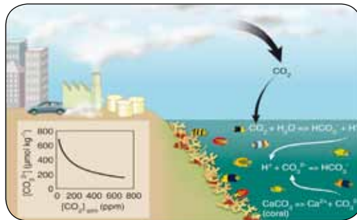
Fig. 2.1 Ocean acidification involves the dissolution of carbon dioxide in the ocean, where it forms a carbonic acid (H 2 CO 3 ). The acid converts carbonate ions into bicarbonate, removing the carbonate building blocks shellfish and other organism need to generate their shells. The net effect on marine calcifiers such as reef building corals is that they slowly fail to calcify. If concentrations get too high, ecosystems such as coral reefs may begin to crumble and dissolved.
